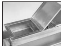
Hilco PTA-40" Pull-Type Aluminum Feltlayer Shown with optional oiler system. Also shown with optional hinged aluminum lid assembly. (Comes standard with side vat covers and baffle setup.) Weight: 121 lbs.
